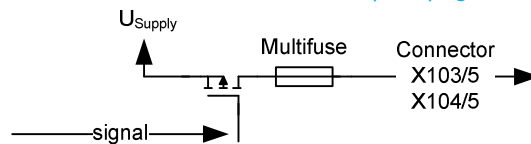
Figure 25: schematic of digital output 1
