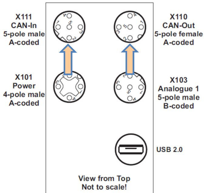
Figure 29: Connect the CAN interface
