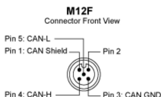
Figure 3 : Connection example
