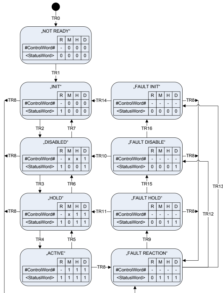
Figure 10: Device state machine
