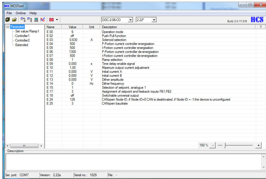
Figure 31: Parameter with HCSTool
