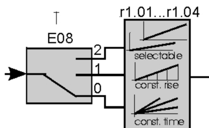
Figure 16: Object 0x6330..0x6336: Ramp function E08 r1.01..r1.04
