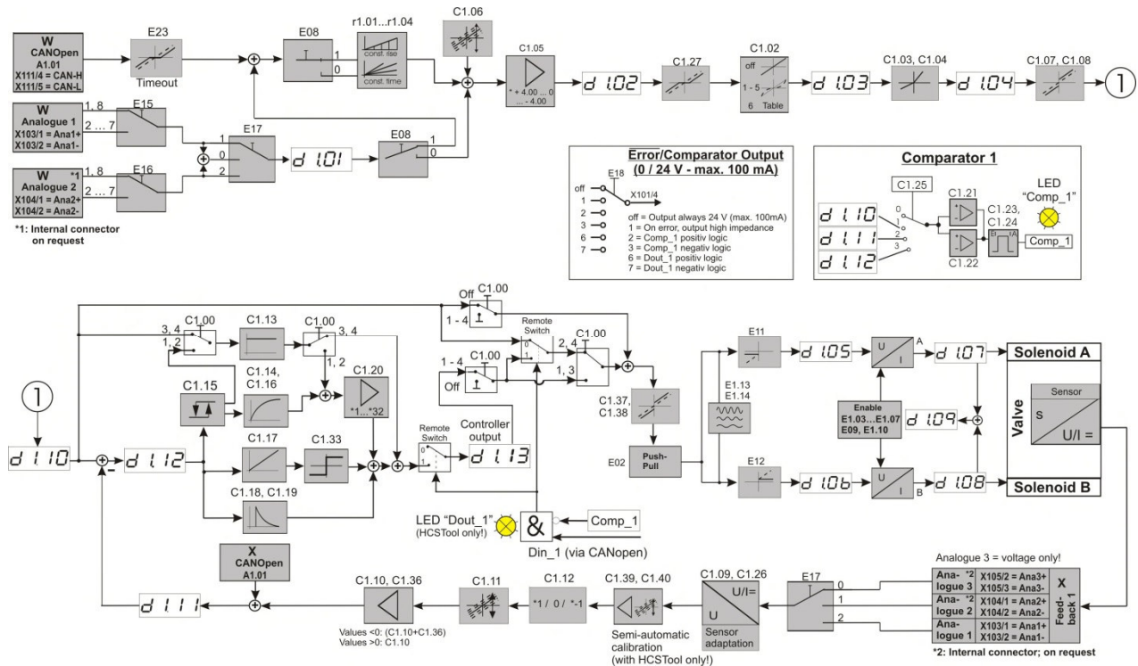
Figure 12: Block diagram mode 3
