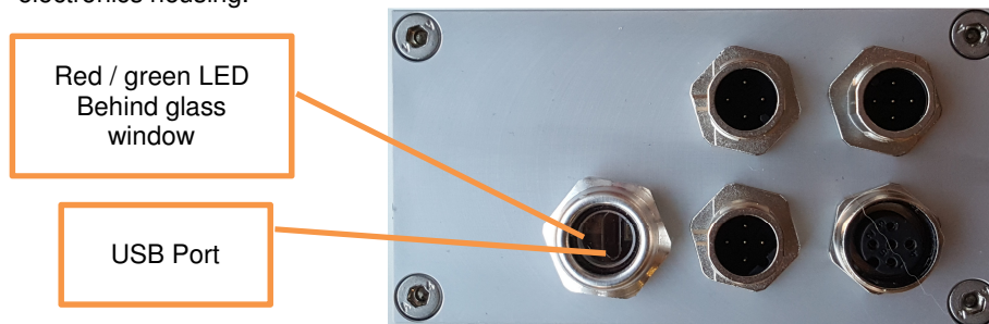
Figure 26: Top view, status LEDs and USB port
