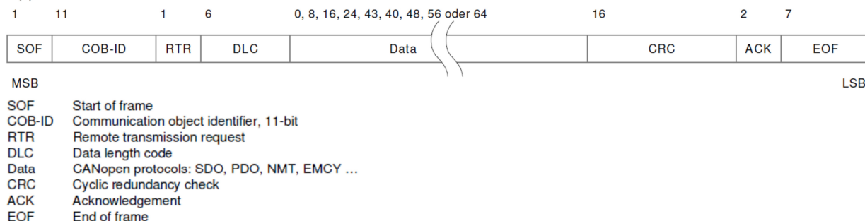
Figure 8: CAN data link layer
