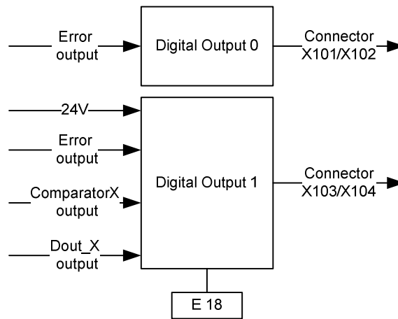
Figure 22: Digital outputs
