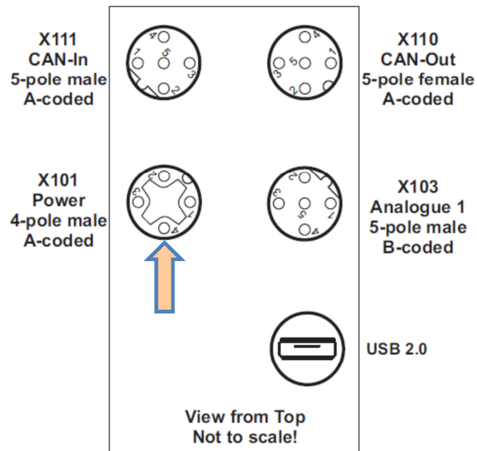
Figure 30: Connect the power to the ODC
