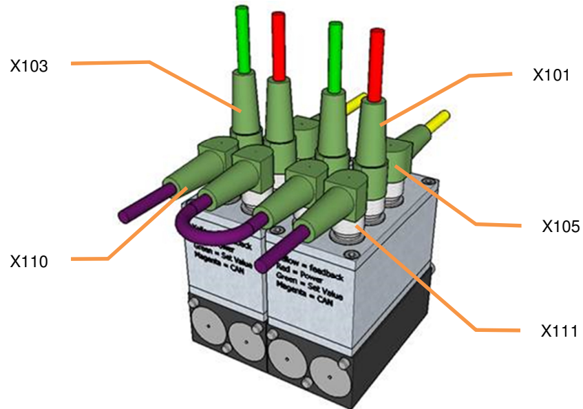
Figure 4: Connection example, Top connection
