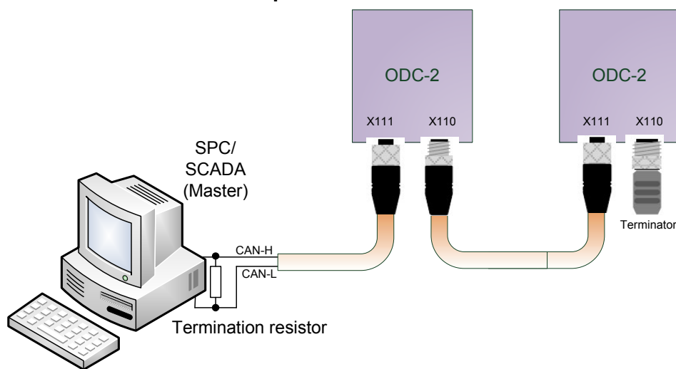
Figure 7: Connection example with termination
