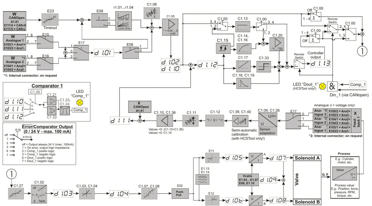
Figure 13: Block diagram mode 4
