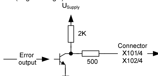
Figure 23: schematic of digital output 0
