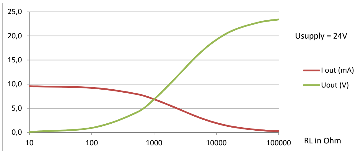
Figure 24: Output high, voltage and current curve at 24V supply
