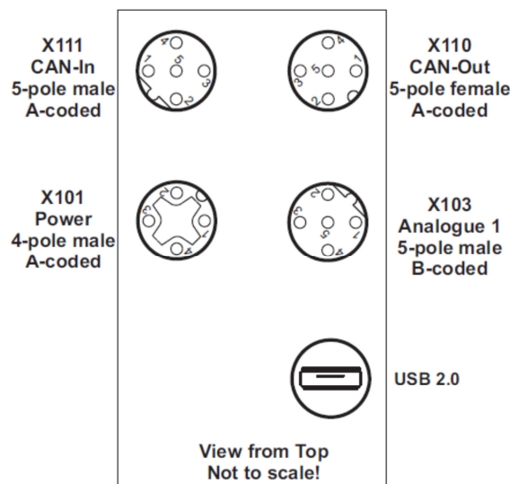
Figure 2 : Connector position layout
