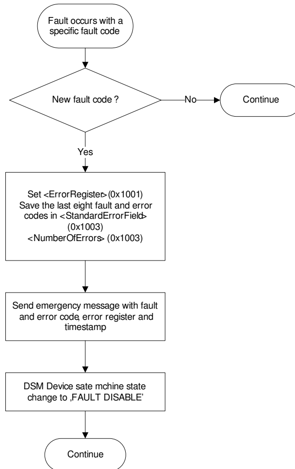
Figure 18: Fault reaction flow chart
