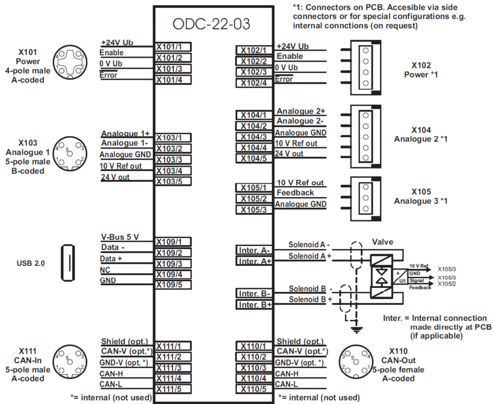
Figure 1 : Connection diagram
