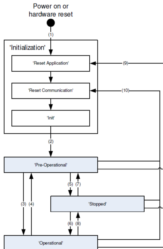
Figure 9: CANopen network state machine (CSM)
