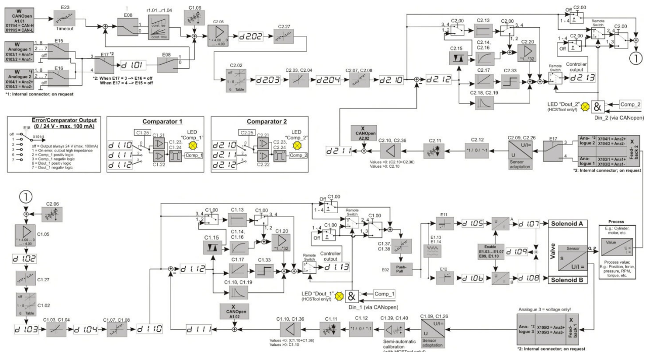
Figure 14: Block diagram mode 6
