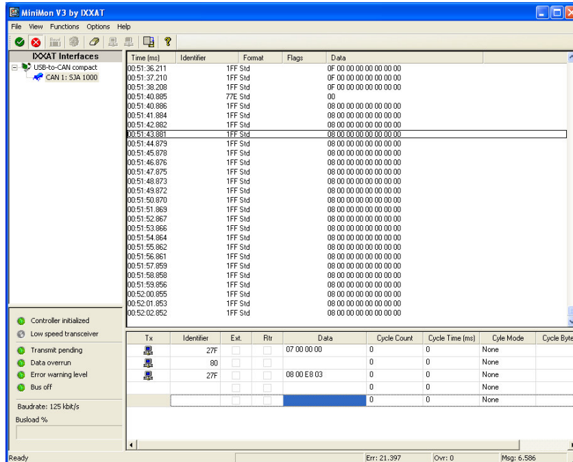
Figure 32: Logging the CAN data transmission
