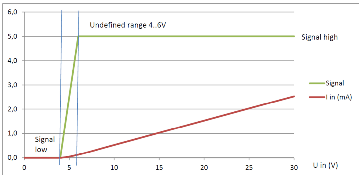
Figure 21: Input Signal curve
