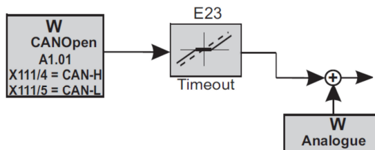
Figure 15: Object 0x6300: Setpoint A1.01
