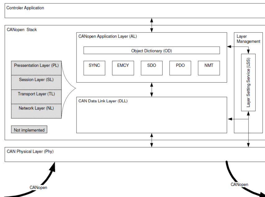
Figure 6: CANopen slave reference model
