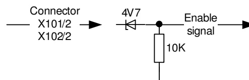
Figure 20: schematic of digital input 0
