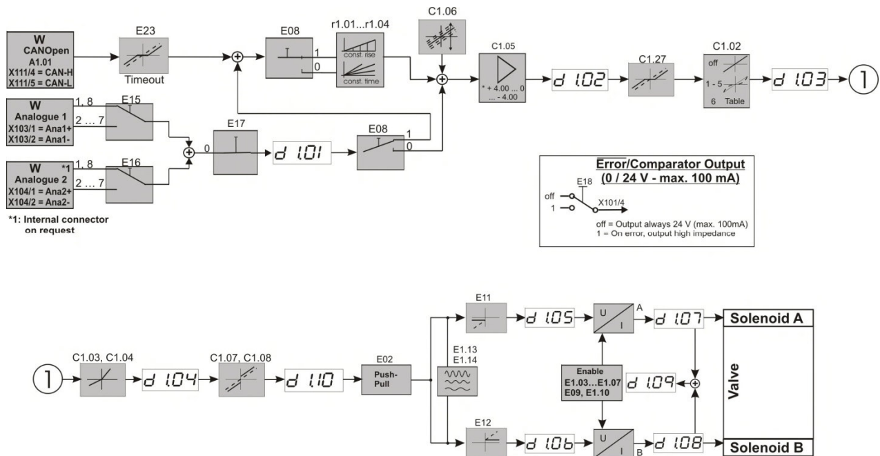
Figure 11: Block diagram mode 1
